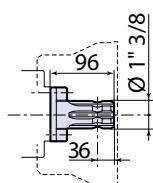
Cardano 1" \frac{3}{8} 1" \frac{3}{8} universal shaft
