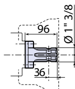
Cardano 1" 3/8 1" 3/8 universal shaft
