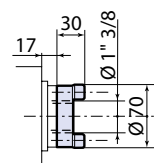
Femmina 1" 3/8 1" 3/8 female
